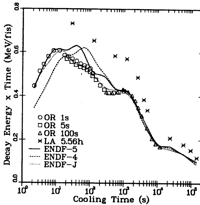
Fig. 140. Comparison of ^{239}\text{Pu} thermal beta fits with experiment, total over all groups.
