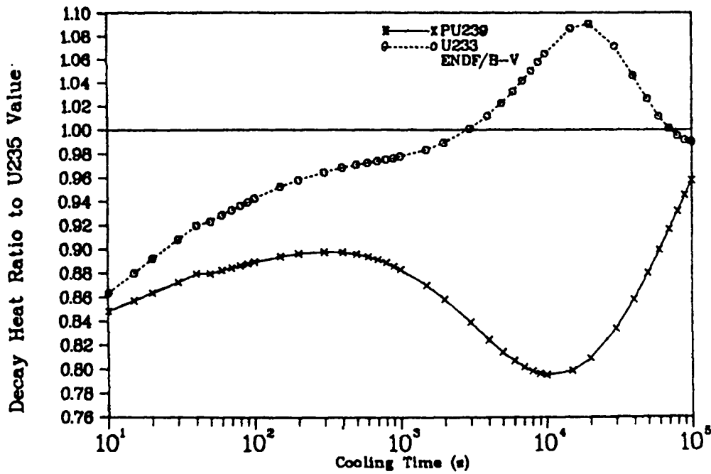
Fig. 14. Ratio of calculated PU239 and U233 to U235 decay heat for 2 \times 10^4 irradiation at constant flux.
