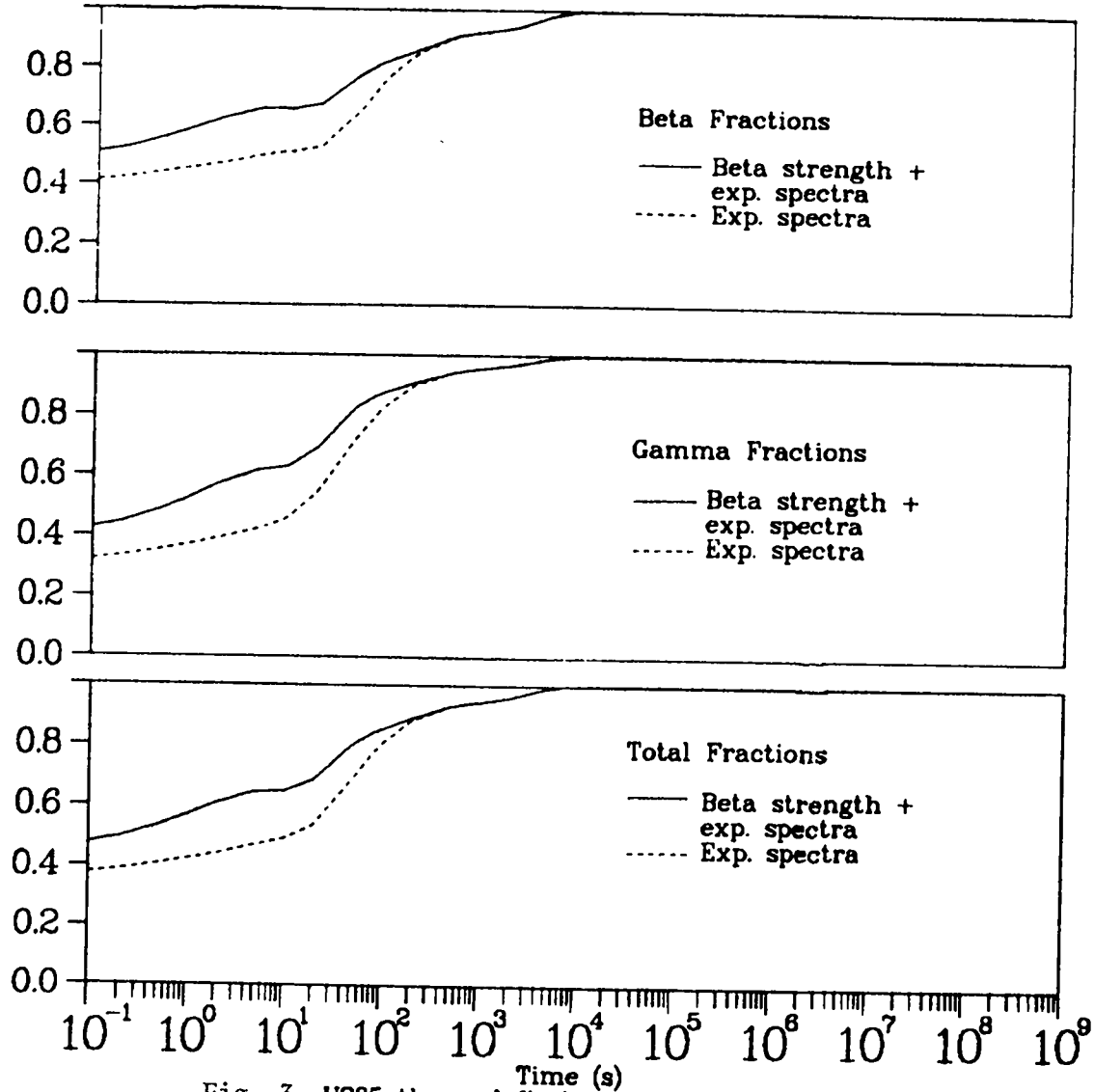
Fig. 3. U235 thermal fission pulse Fractional energies from experimental data in ENDF/B-V
