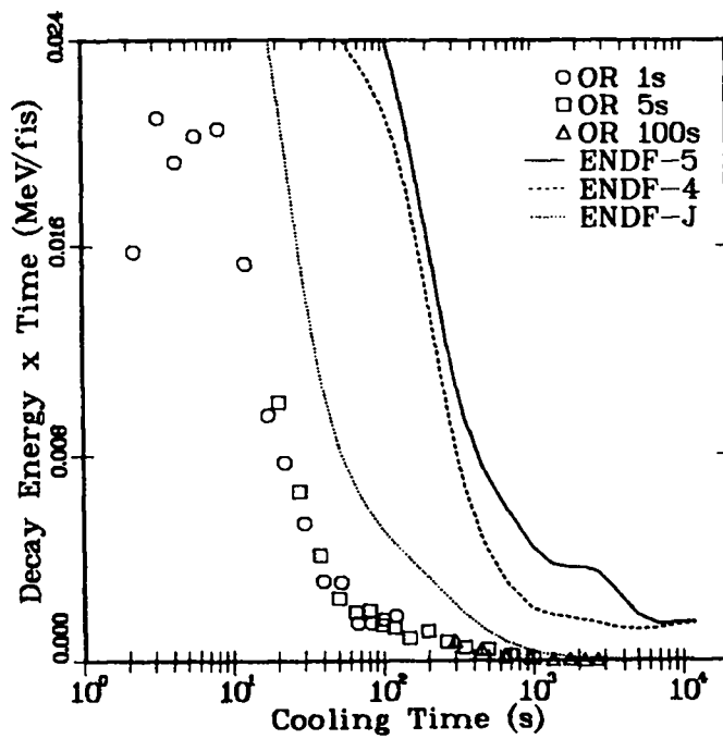
Fig. 138. Comparison of ^{239}\text{Pu} thermal beta-fits with experiment, Group 17.
