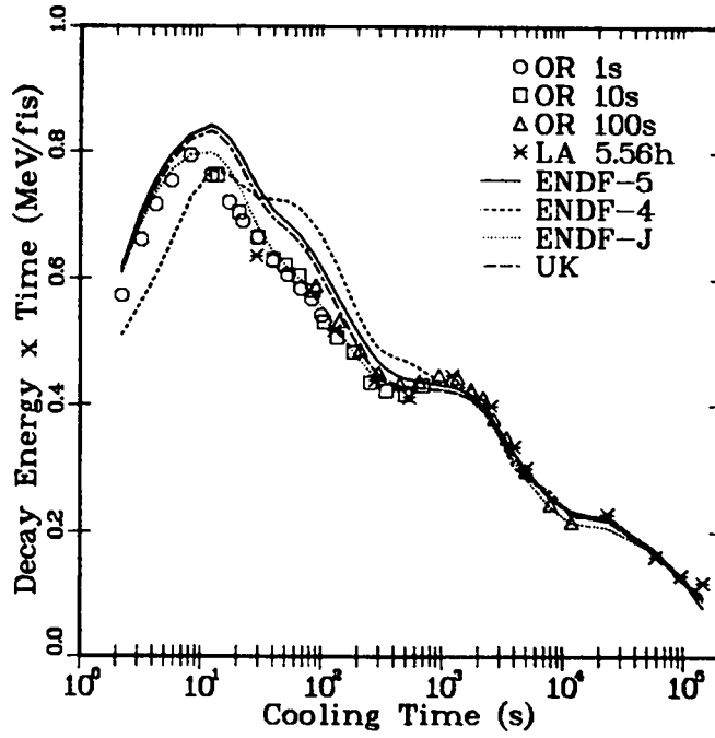
Fig. 139. Comparison of ^{235}\text{U} thermal beta fits with experiment, total over all groups.
